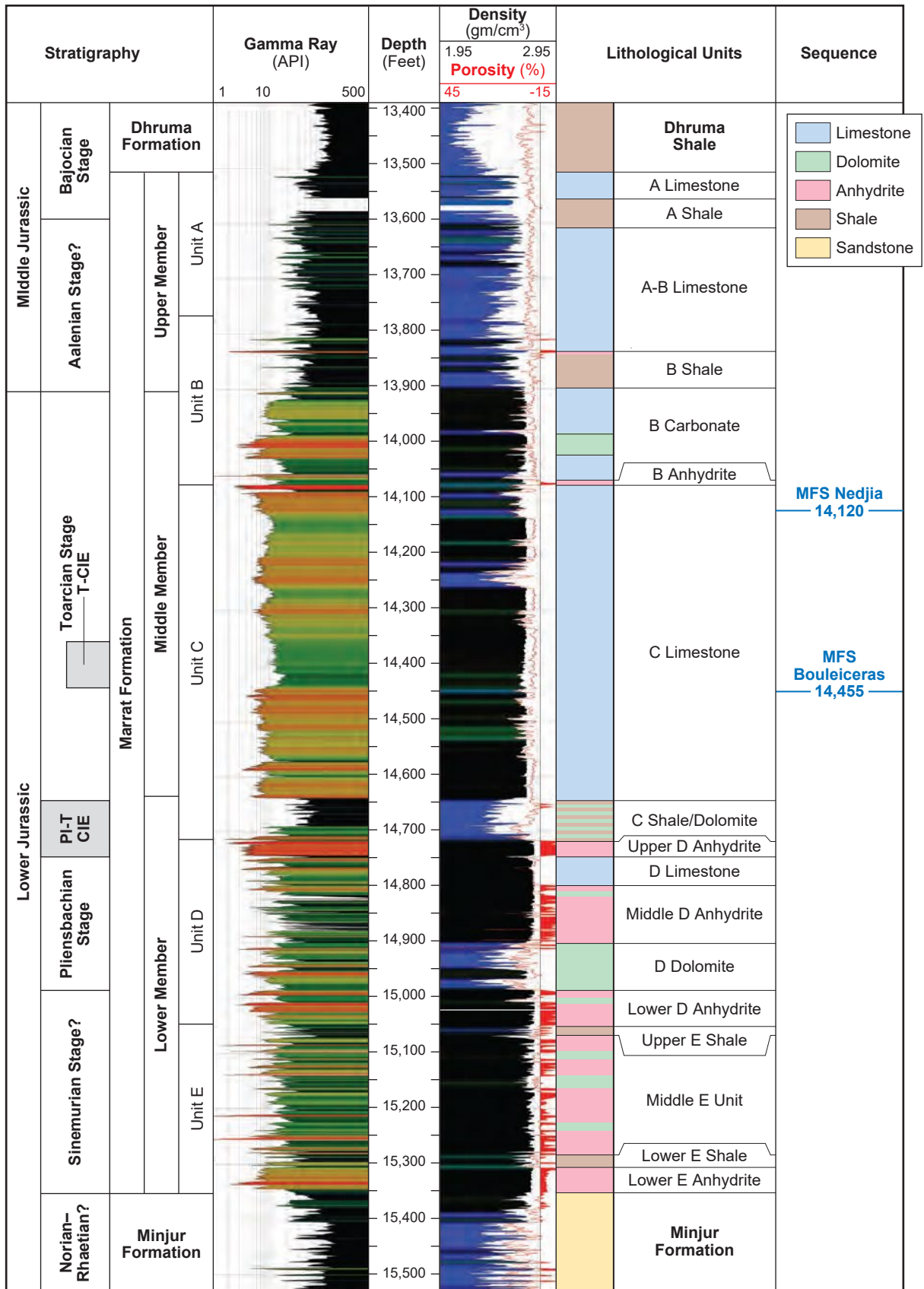
Figure 11: The Marrat Formation in Kuwait is defined in the Minagish-27 borehole (Yousif and Nouman, 1997).
